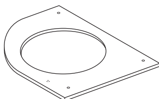
4-480X400X12mm(1pc)
